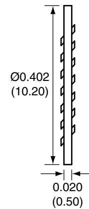
WASHER
